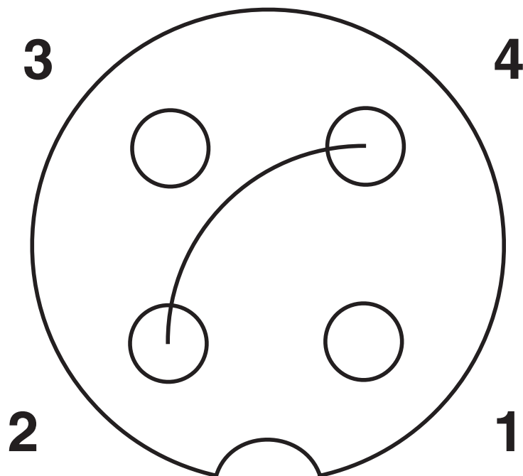
Schematic diagram
