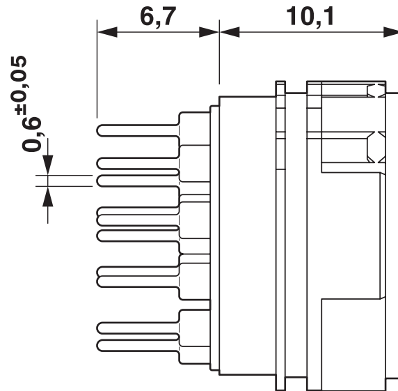
Dimensional drawing
