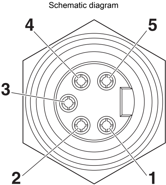
Pin assignment, socket, 7/8"-16UNF, 5-pos., view of female side (reference image)
