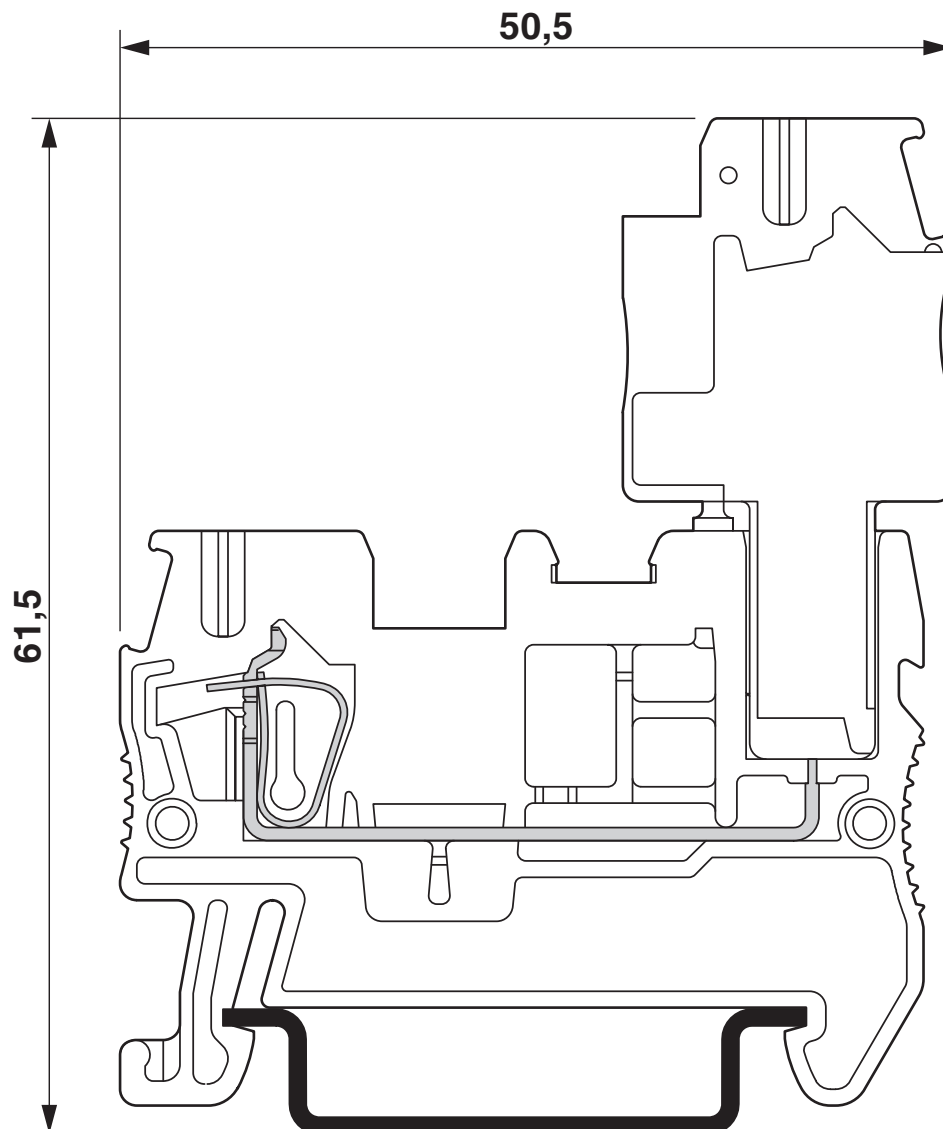
Dimensional drawing
