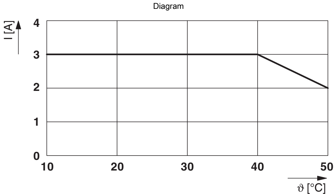
Derating curve for limiting continuous current
