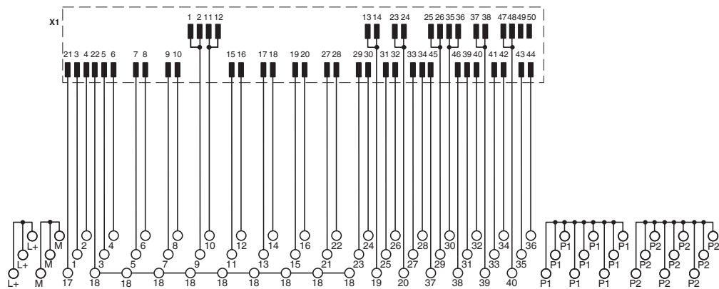
Circuit diagram
