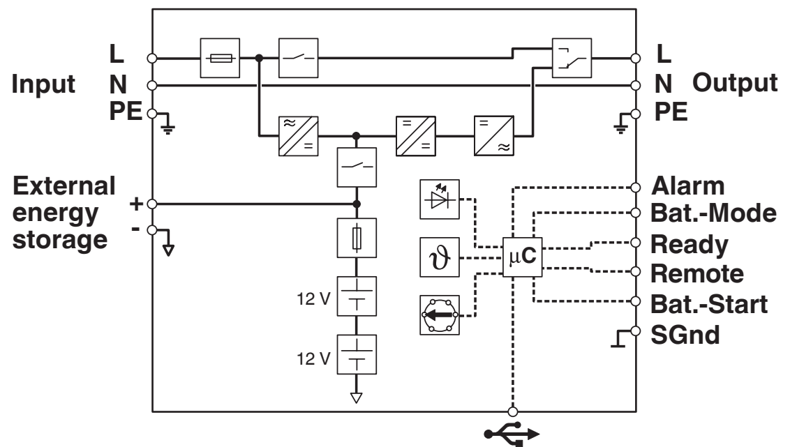
Block diagram
