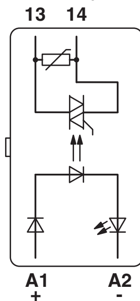
Circuit diagram
