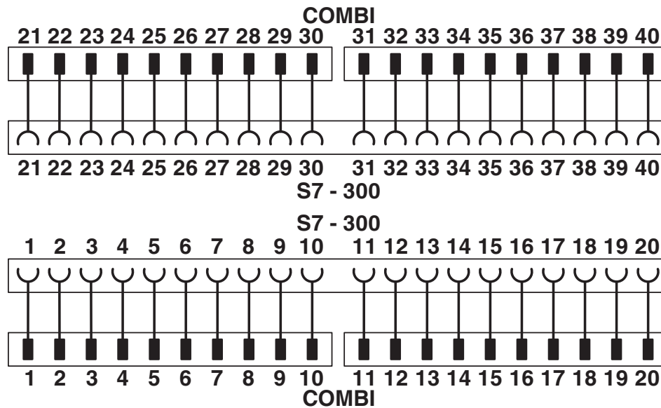
Circuit diagram
