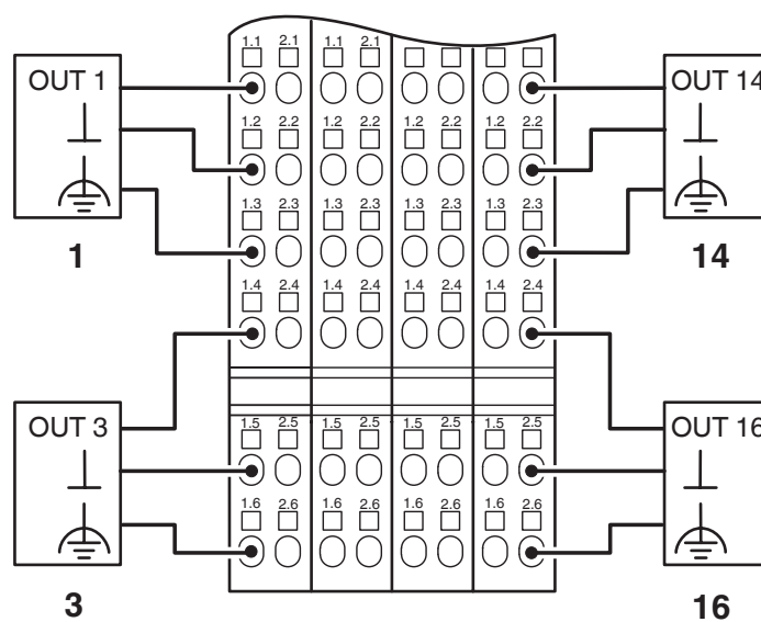
Connection diagram
