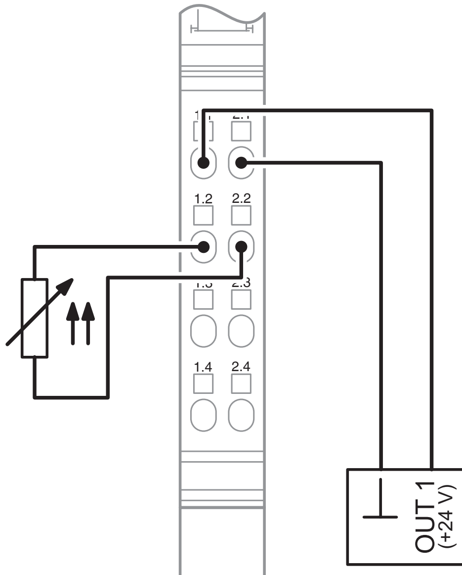
Connection diagram
