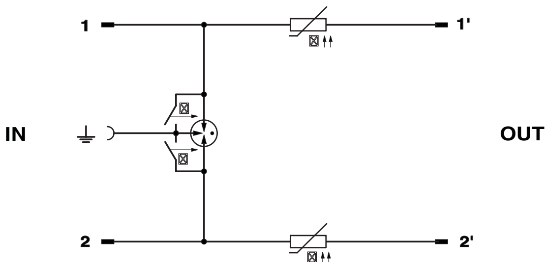
Circuit diagram
