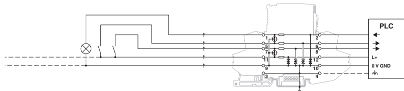
Application drawing
