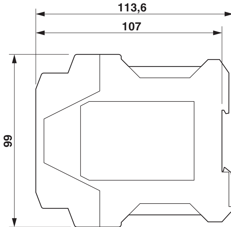
Dimensional drawing
