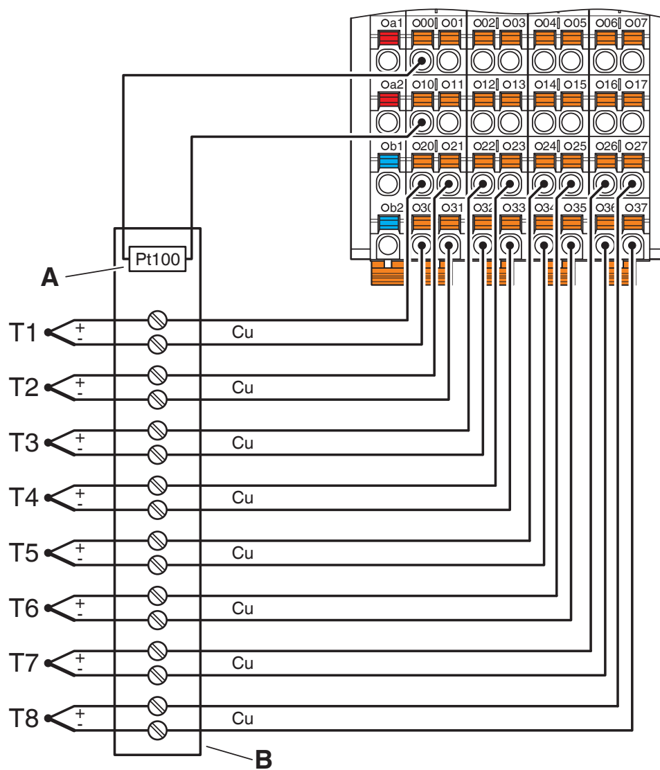
Connection diagram
