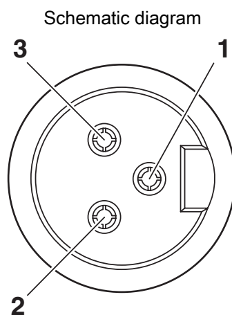
Pin assignment, socket, 1-3/8"-16UNF, 3-pos., view of female side
