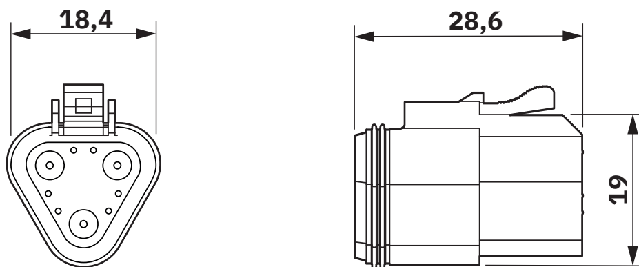
Dimensional drawing
