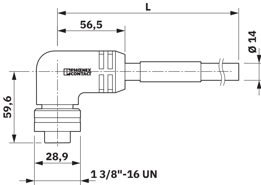
Dimensional drawing
