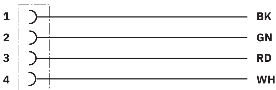
Contact assignment of 1-3/8" plugs/sockets
