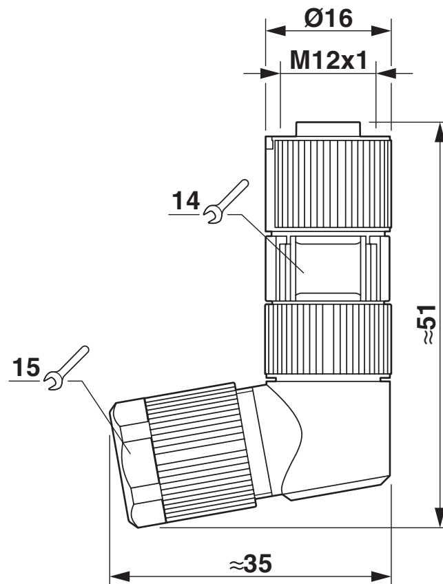
Dimensional drawing
