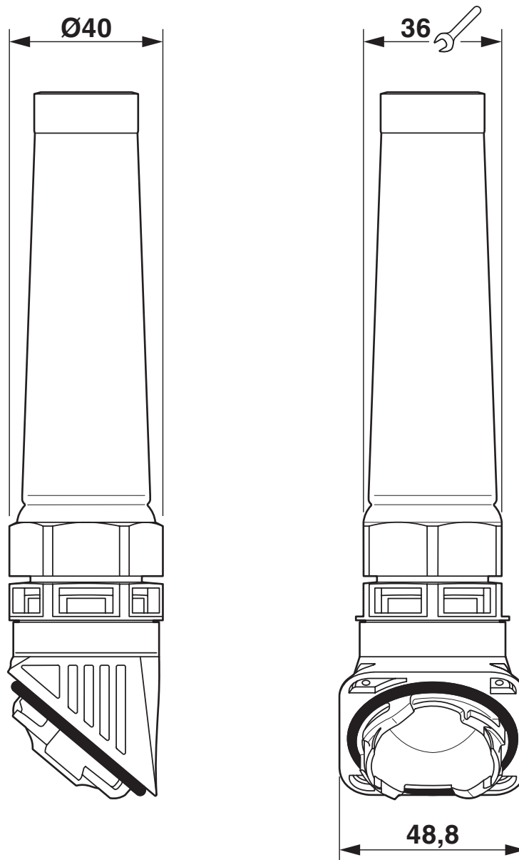
Dimensional drawing
