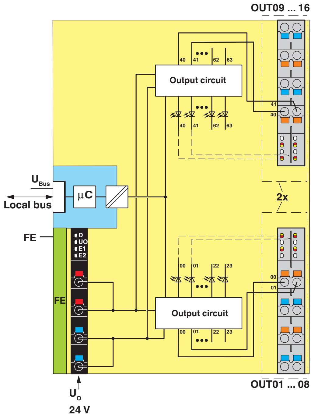
Block diagram
