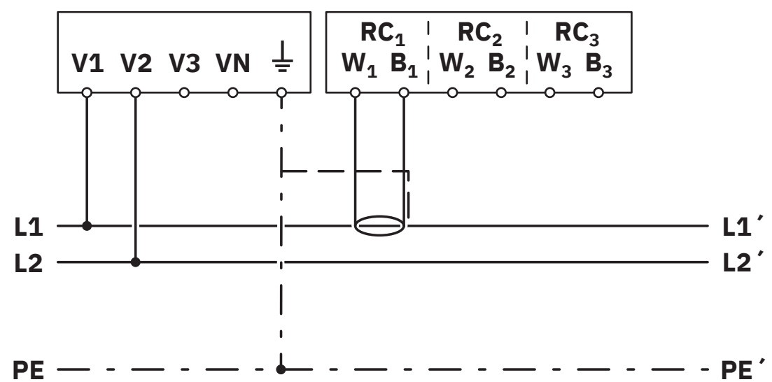
Connection diagram
