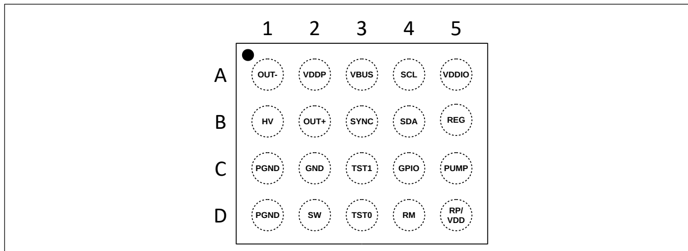
Figure 3: WLCSP 20B 2.1mm × 1.7mm package (TOP VIEW; NOT TO SCALE)
