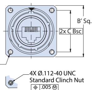
CM & CS - Wall Mount Receptacle with Metric/Std Clinch Nuts (Mating Face)
