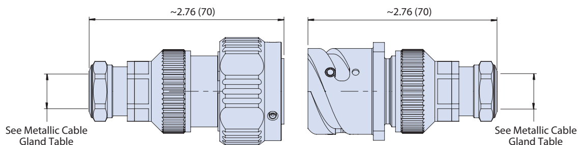
Plug and Receptacle without Pigtail
