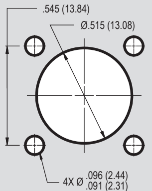
SQUARE FLANGE RECEPTACLE
