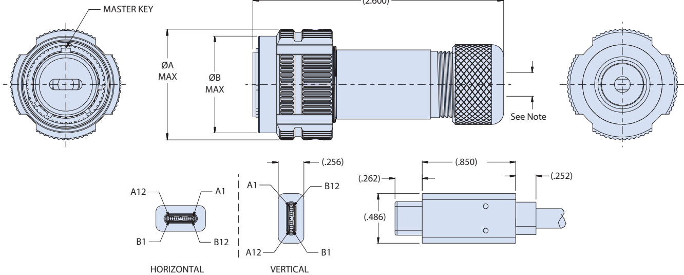
Recommended USB 3.1 Type C Plug Overmold Design
