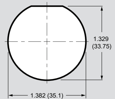
JAM NUT MOUNT
