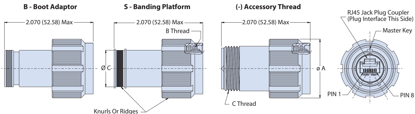
Plug Dimensions
