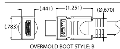
OVERMOLD BOOT STYLE: B
