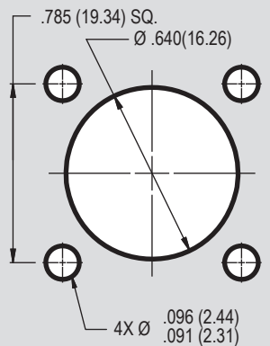
SQUARE FLANGE RECEPTACLE
