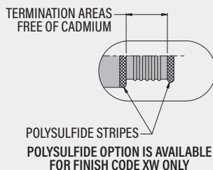
FIGURE 1 POLYSULFIDE OPTION
