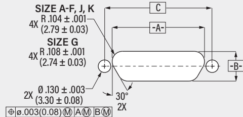
PANEL CUTOUT FOR SERIES 790 SHELL SIZES A-G, J, K
