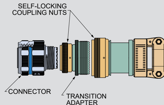
Style 2 Backshell
