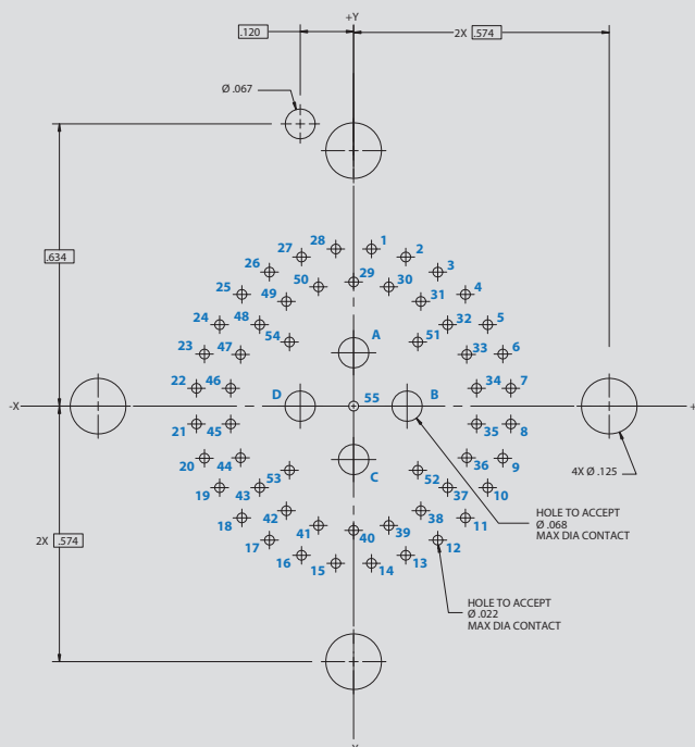
4x #16 and 55x #22HD Contacts
