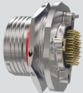
PCB Jam-Nut Receptacle, with Threaded Standoffs CODE RED 806-028 Page 109
