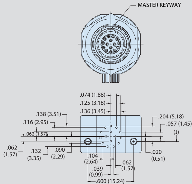
ARRANGEMENT NO. 10-15 15 X #22HD CONTACTS PIN FACE SHOWN (SOCKET FACE OPPOSITE)
