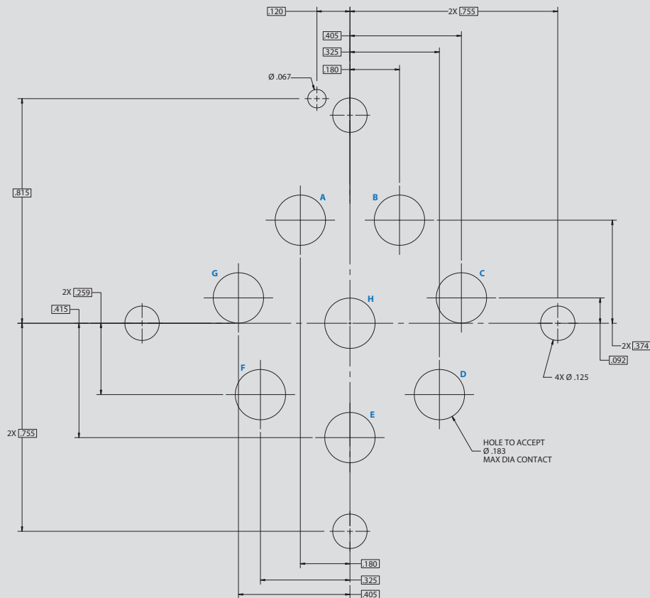
Arrangement No. 24-8 8x #8 EI Ochito Contacts
