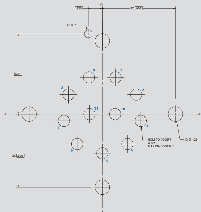
Arrangement No. 20-11 11x #12 Contacts
