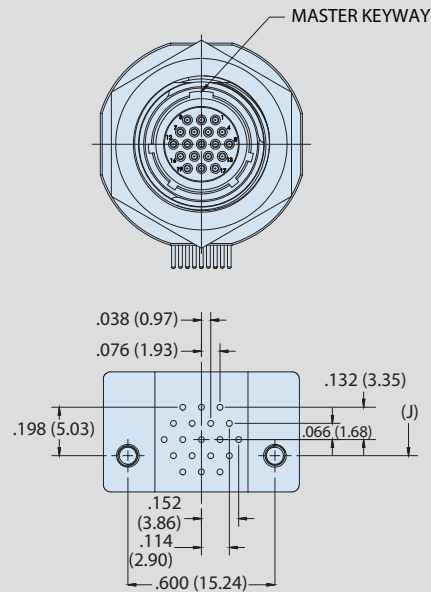
ARRANGEMENT NO. 11-19 19 X #22HD CONTACTS PIN FACE SHOWN (SOCKET FACE OPPOSITE)
