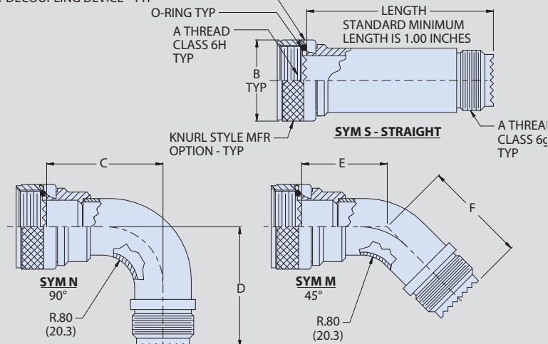
ANTI-DECOUPLING DEVICE - TYP
