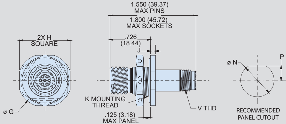
806-087-07 Jam-Nut Mount Receptacle Dimensions
