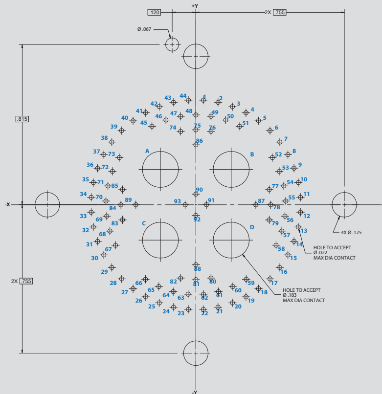
93 #22HD and 4 #8 Contacts
