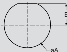
Jam-Nut Cutout
