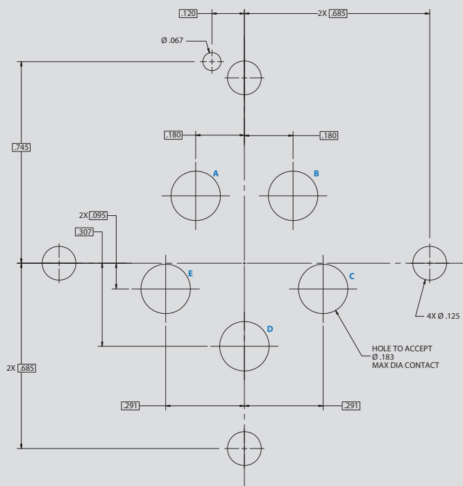
Arrangement No. 22-5 5x #8 Contacts
