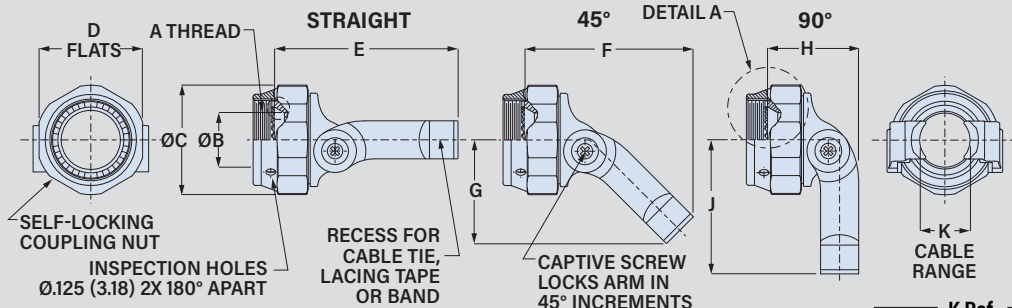
BANDING ADAPTER WITH OPTIONAL T-SLOTS
