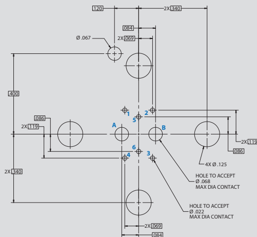
Arrangement No. 10-8A 2x #16 and 6x #22HD Contacts
