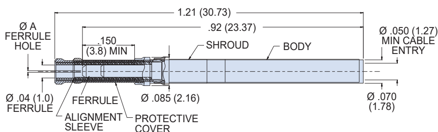
#20HD Socket Terminus 181-135
