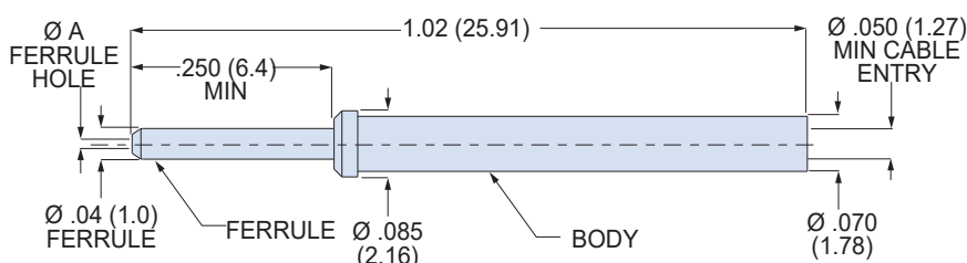
#20HD Socket Terminus 181-135
