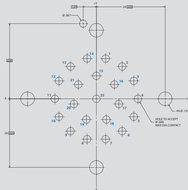
Arrangement No. 20-22 22x #16 Contacts
