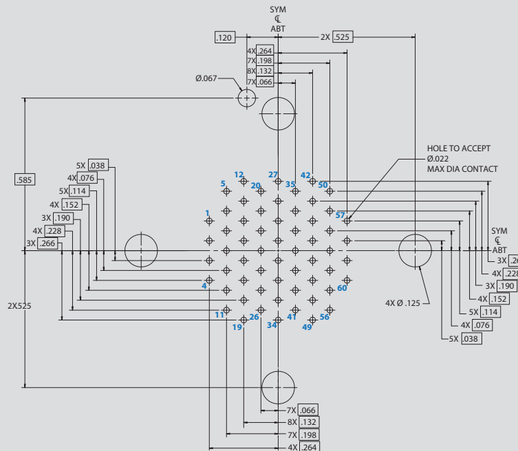
Arrangement No. 16-60 60x #22HD Contacts
