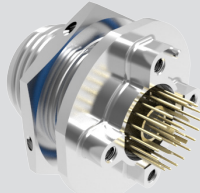
PCB Jam-Nut Receptacle, High-Speed El Ochito® CODE RED 806-043 Page 111
