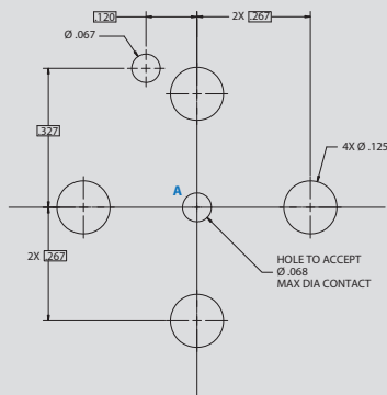
Arrangement No. 8-1 1x #16 Contacts
