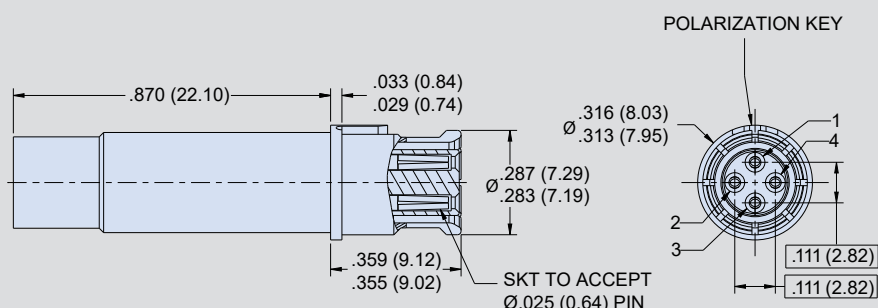
Socket Contact 854-048
