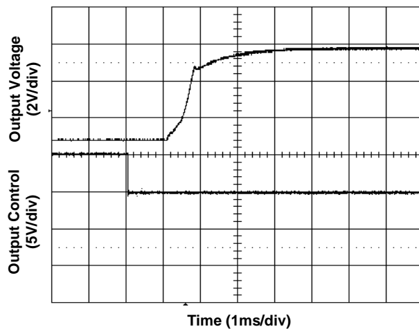
Figure 4. Start-Up from Enable Control (Typical input voltage and full load)
