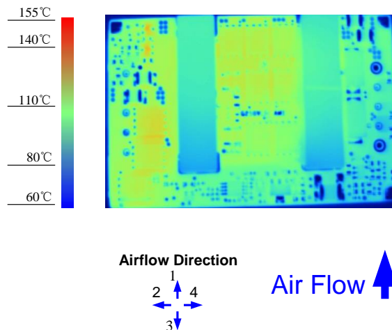
Figure 9. Thermal Image for Airflow Direction 1 (25.5A output, 55°C ambient, 200 LFM, typical Vin, open frame, unit soldered onto a fixture board.)
