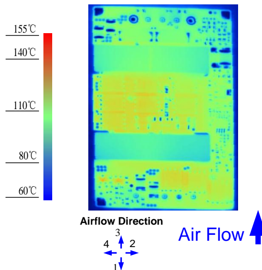
Figure 11. Thermal Image for Airflow Direction 3 (24.3A output, 55°C ambient, 200 LFM, typical Vin, open frame, unit soldered onto a fixture board.)
