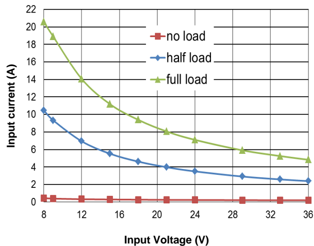
Figure 3. Input Characteristics
