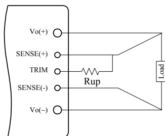
Figure 16 Circuit to Increase Output Voltage
