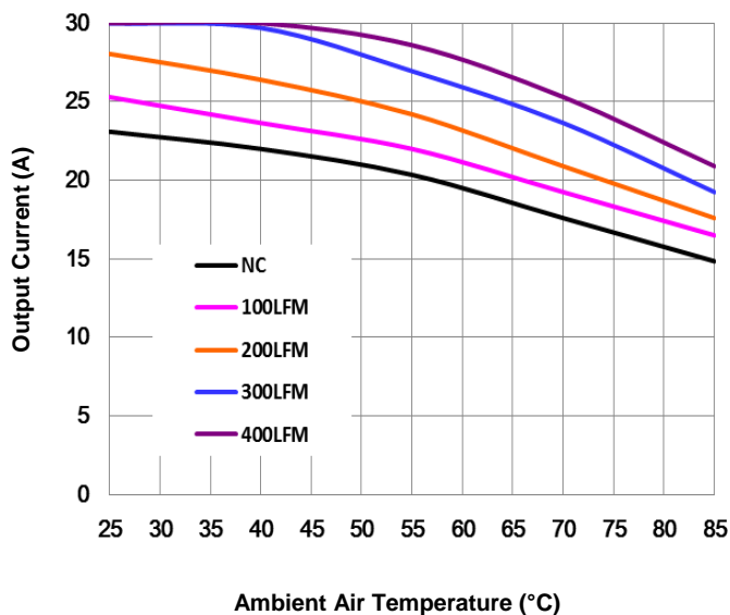
Figure 10. Current Derating Curve for Airflow Direction 3 (Ref. Figure.11 for Airflow Direction; typical Vin, open frame, unit soldered onto a fixture board.)
