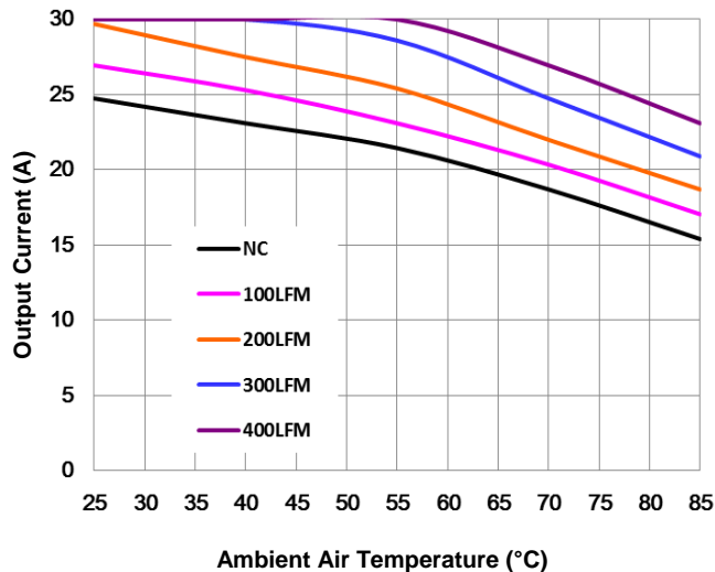
Figure 8. Current Derating Curve for Airflow Direction 1 (Ref. Figure. 9 for Airflow Direction; typical Vin, open frame, unit soldered onto a fixture board.)
