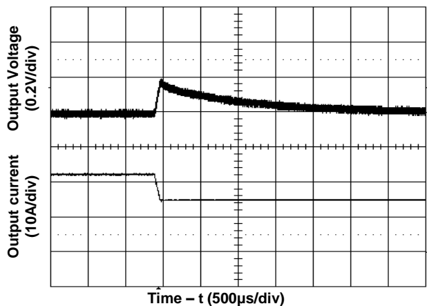
Figure 7 Transient Load Response (Typical Vin, 75% to 50% full load step at a slew rate 0.1A/µs)
