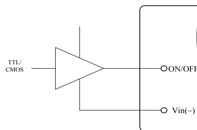
Figure 14. Direct Logic Drive
