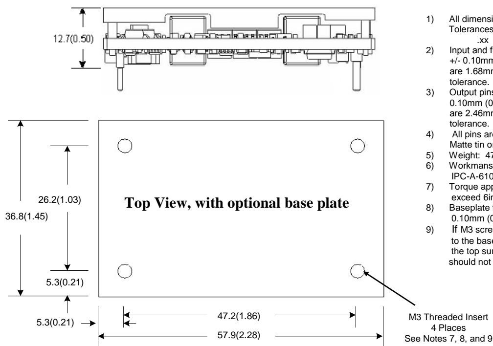
Figure 19. Converter with optional baseplate
