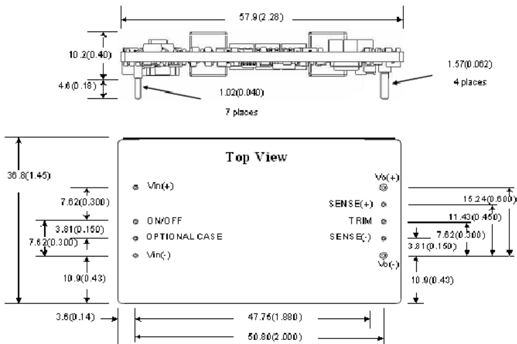
Figure 18. Open Frame Converter
