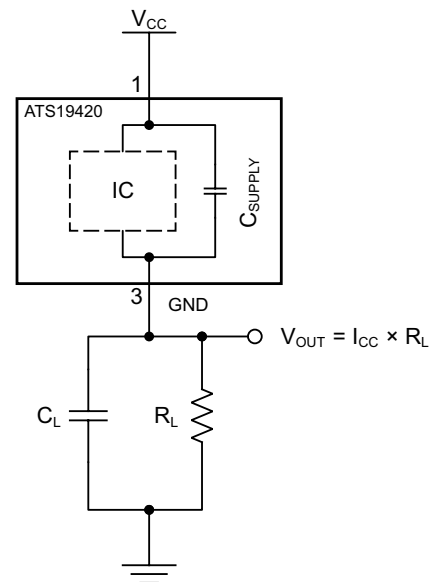
Figure 1: Typical Application Circuit
