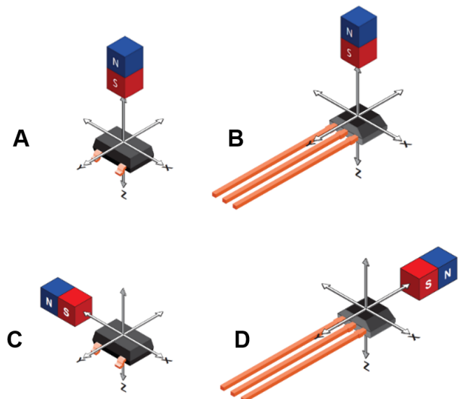
Figure 6: Magnetic Sensing Orientations APS11700 LH (Panel A), APS11700 UA (Panel B), APS11760 LH (Panel C), and APS11760 UA (Panel D)
