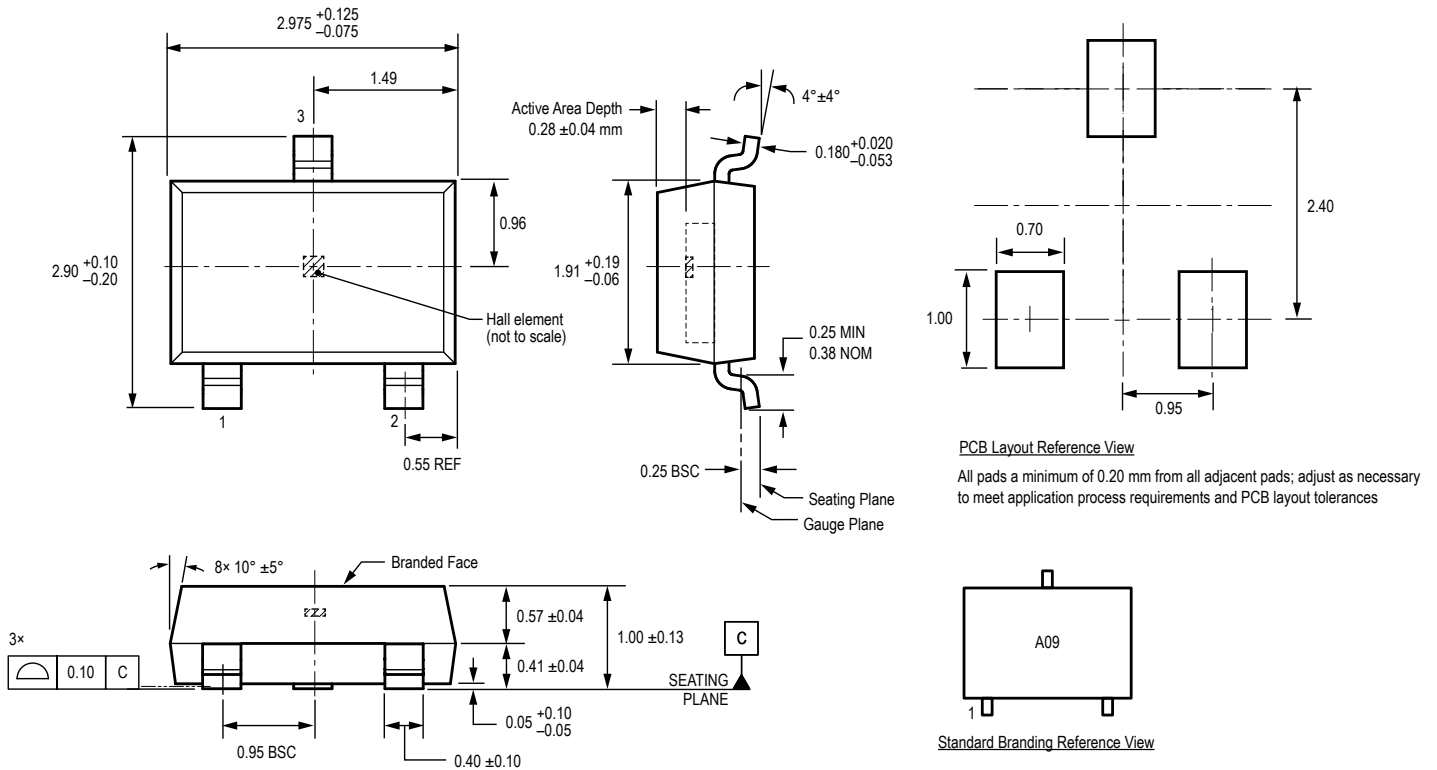
Figure 9: Package LH, 3-Pin SMD (SOT23W), APS11700
