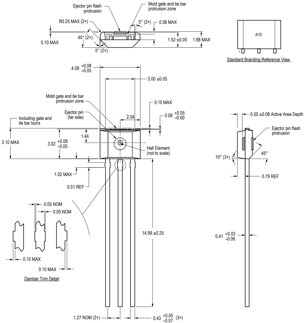
Figure 10: Package UA, 3-Pin SIP, APS11700
