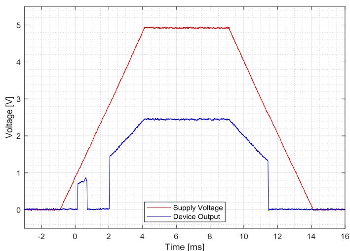
Figure 2: Power-On Profile
