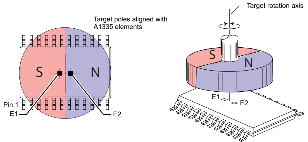
Figure 12: Orientation of Magnet Relative to Primary Die and Secondary Die
