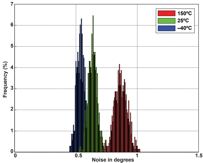
Figure 24: Noise Distribution over Temperature (3 Sigma, 300 G)
