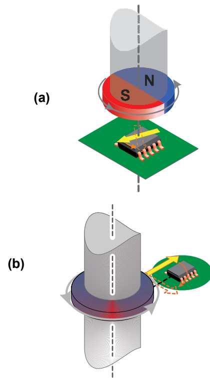
Figure 13: Typical On-Axis (a) and Off-Axis (b) Orientation
