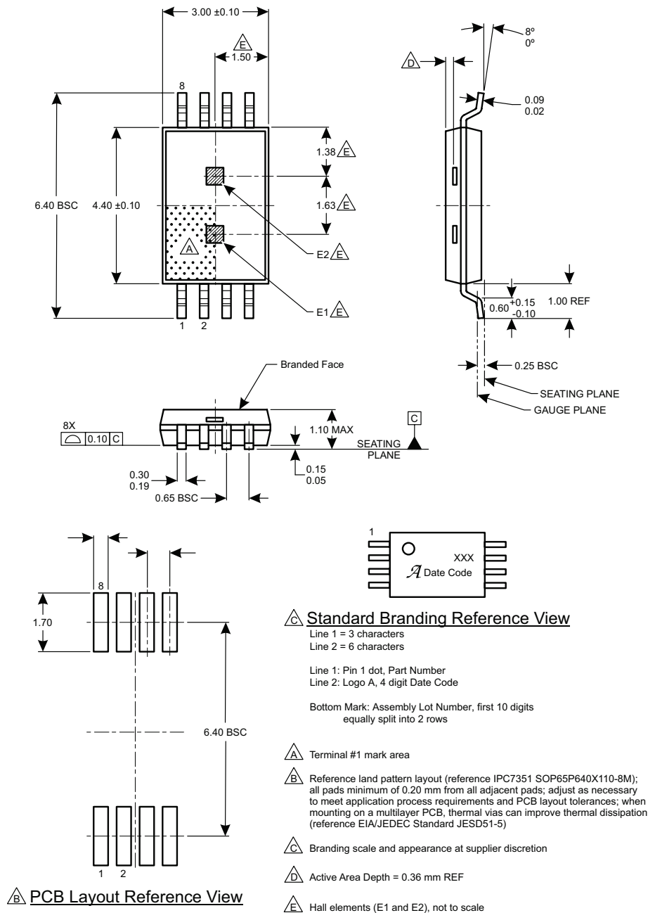
Figure 13: Package LE, 8-Pin TSSOP
