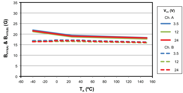
Channel A & B: Average Switchpoint Hysteresis versus Ambient Temperature
