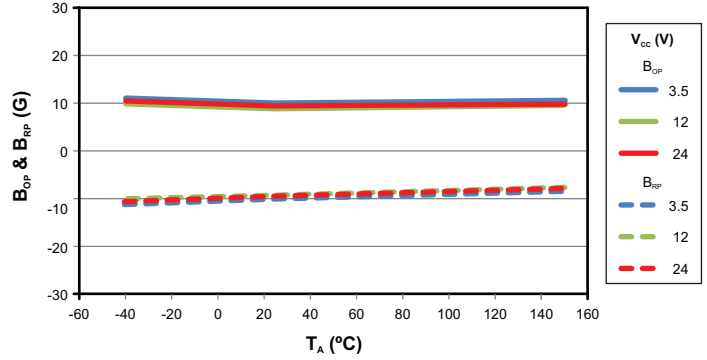
Channel A: Average Operate & Release Points versus Ambient Temperature
