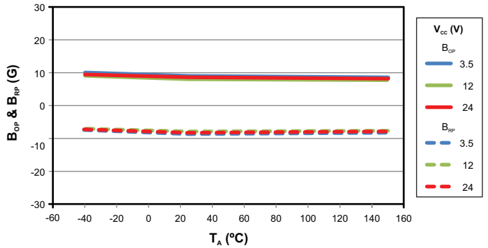
Channel B: Average Operate & Release Points versus Ambient Temperature
