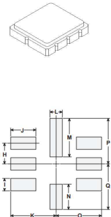
PCB Footprint
