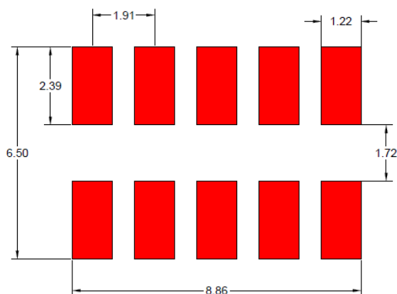
Typical PCB Land Pattern
