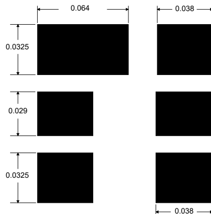
Foot Print Dimensions in Inches
