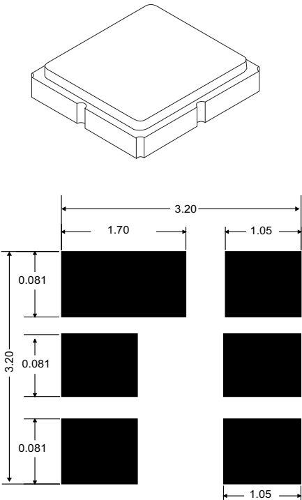
PCB Footprint (in millimeters)
