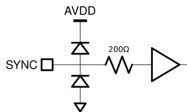
Figure 29: Equivalent SYNC Input Circuit.
