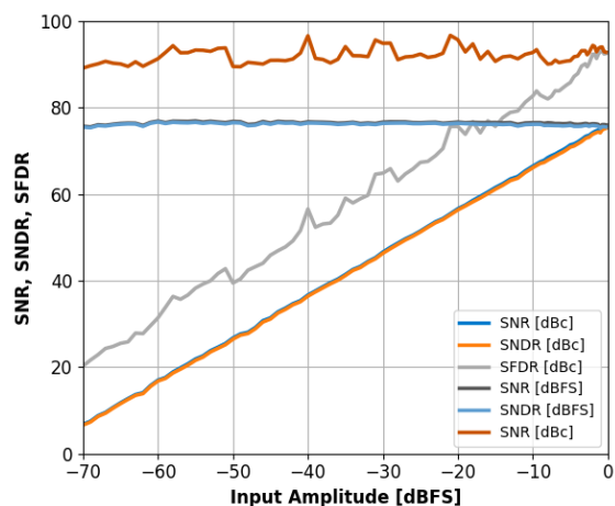
Figure 17: Single-Tone SNR, SNDR and SFDR vs. Input Amplitude with f_{IN}=30.2\text{MHz} .
