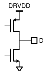
Figure 27: Equivalent Digital Output Circuit.
