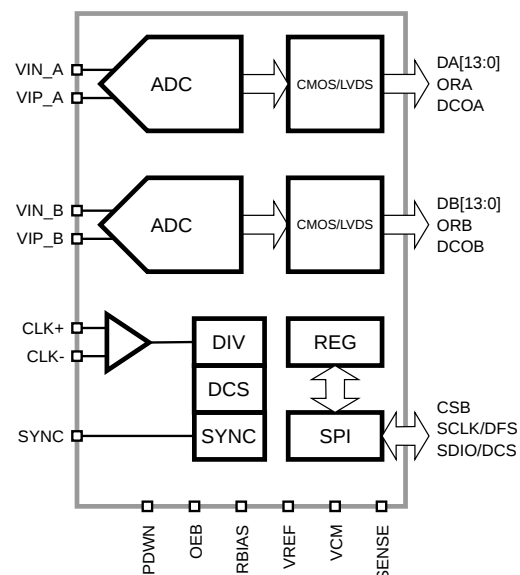
Figure 1: SD9648 Functional Block Diagram.
