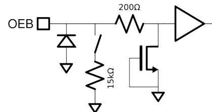
Figure 25: Equivalent OEB Input Circuit.
