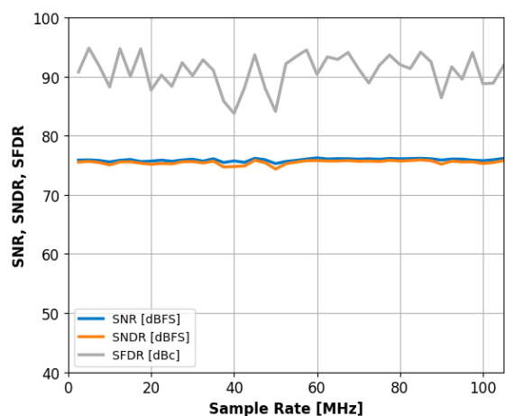
Figure 19: Single-Tone SNR, SNDR and SFDR vs. Sample Rate with f_{IN}=30.2\text{MHz} .
