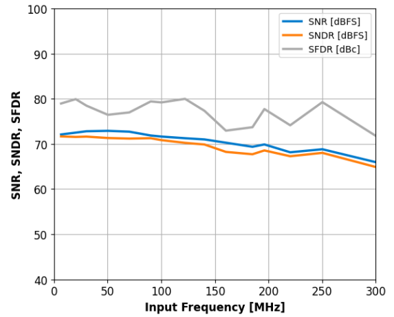
Figure 16: Single-Tone SNR, SNDR and SFDR vs. Input Frequency with f_s=250\text{MHz} .
