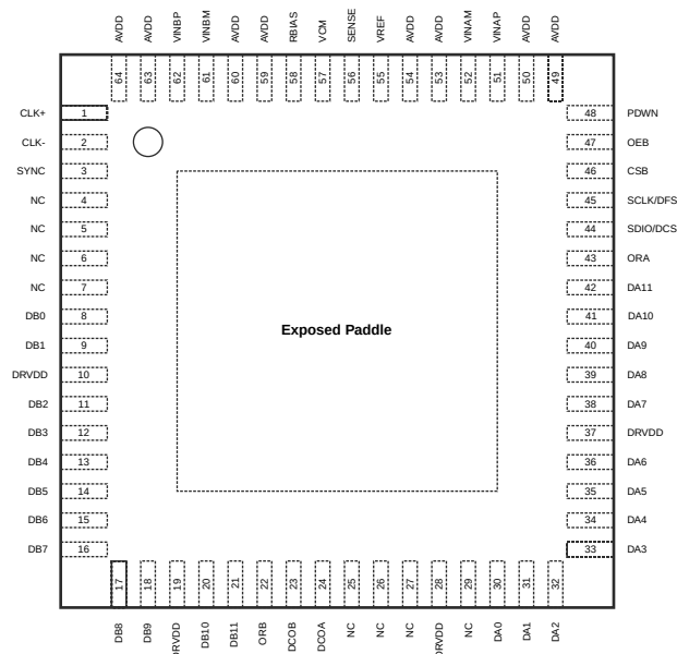
Figure 6: SD9628 Package Top View for Parallel CMOS Configuration.
