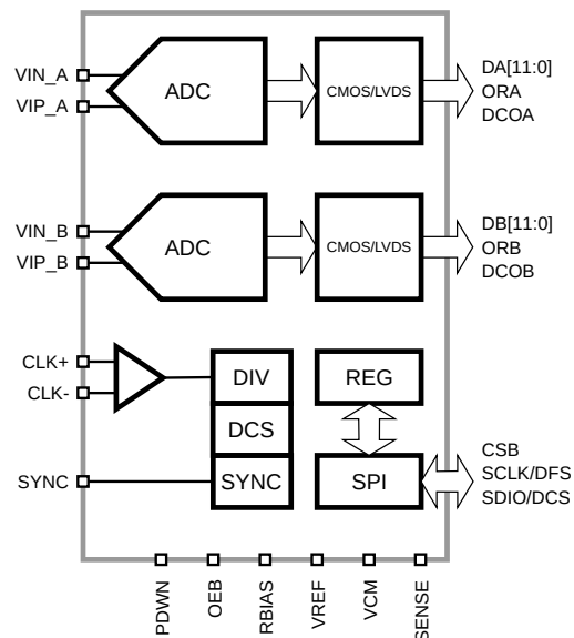
Figure 1: SD9628 Functional Block Diagram.
