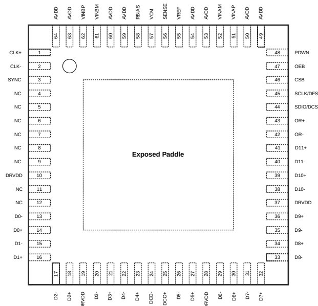
Figure 7: SD9628 Package Top View for Interleaved Parallel LVDS Configuration.
