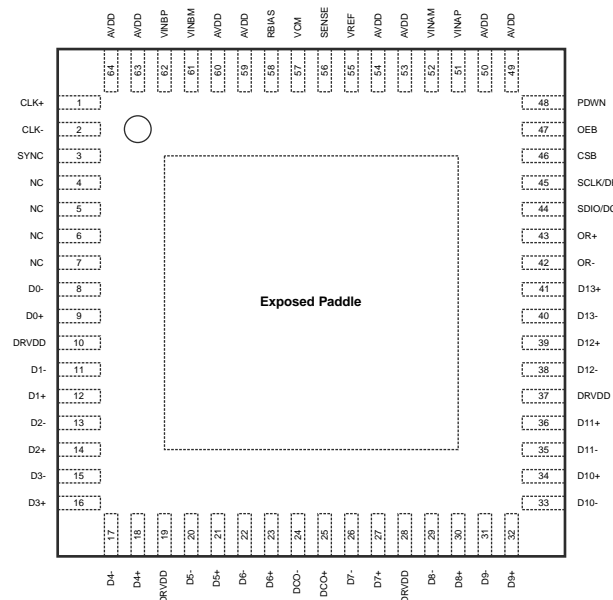
Figure 6: SD9258 Package Top View for Parallel LVDS Configuration.
