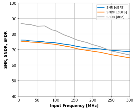
Figure 14: Single-Tone SNR, SNDR and SFDR vs. Input Frequency with f_s=40\text{MHz} .
