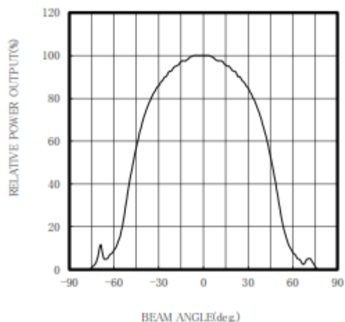
RADIATION PATTERN
