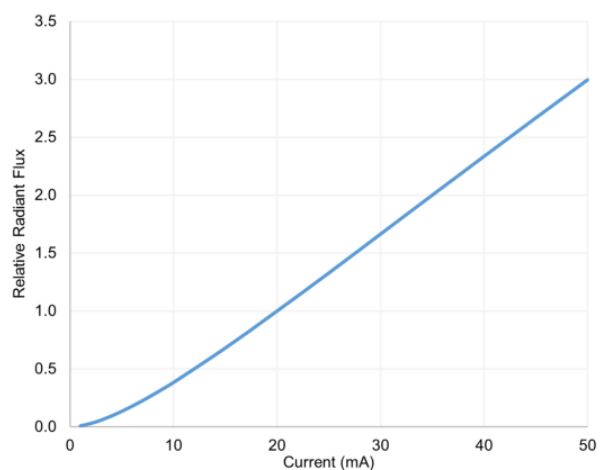
Figure 2. Relative radiant flux vs forward current T_A = 25^\circ\text{C}
