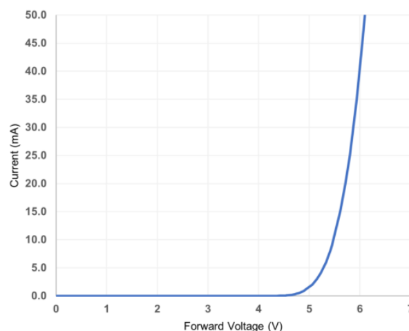
Figure 4. Forward current vs forward voltage T_A = 25^\circ\text{C}
