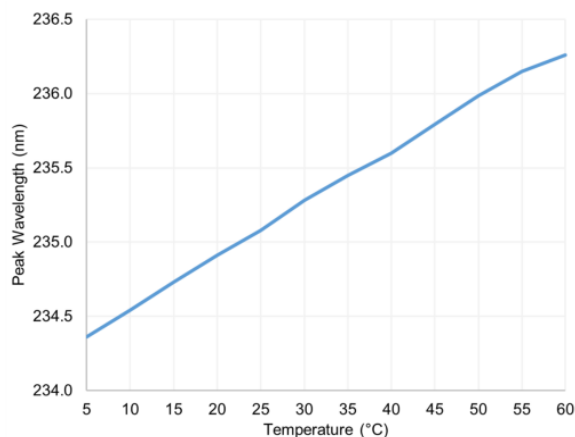
Figure 6. Peak wavelength vs temperature I_F = 20\text{ mA}
