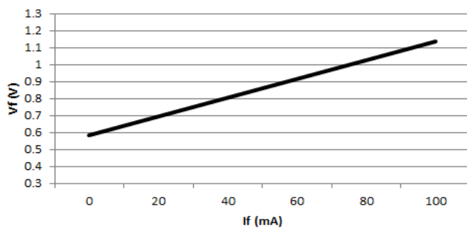
Forward V-I Characteristics
