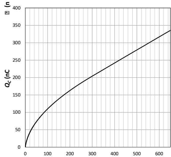
Fig. 7 Capacitive Charge
