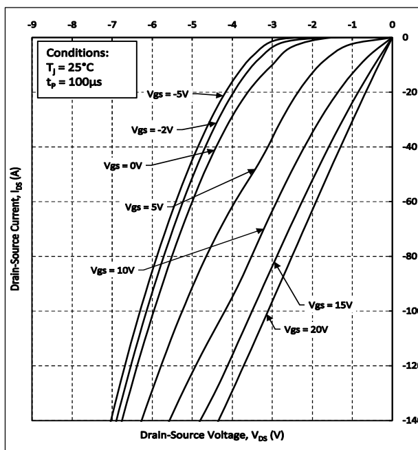
Figure 10. Body Diode Characteristics at T_J = 25^\circ C
