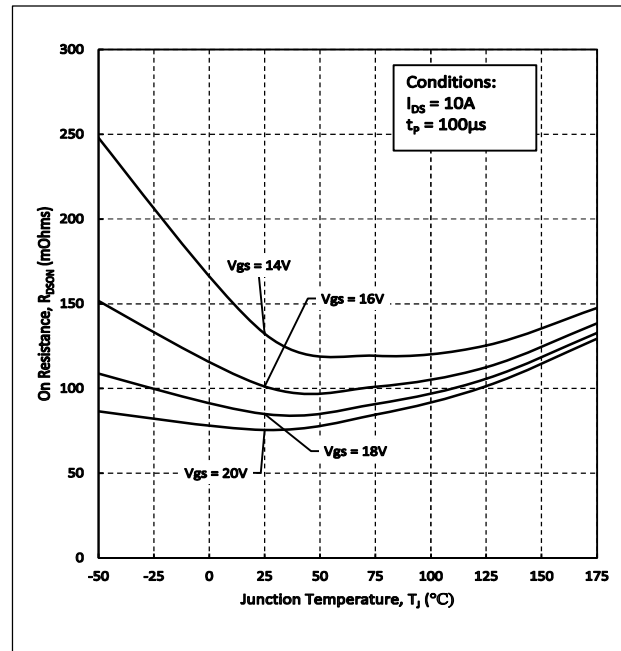
Figure 6. On-Resistance vs. Temperature For Various Gate Voltages
