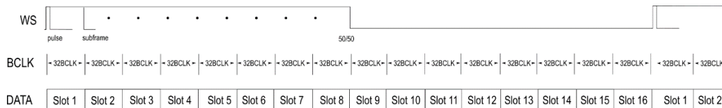
Figure 26 - TDM16 Mode
