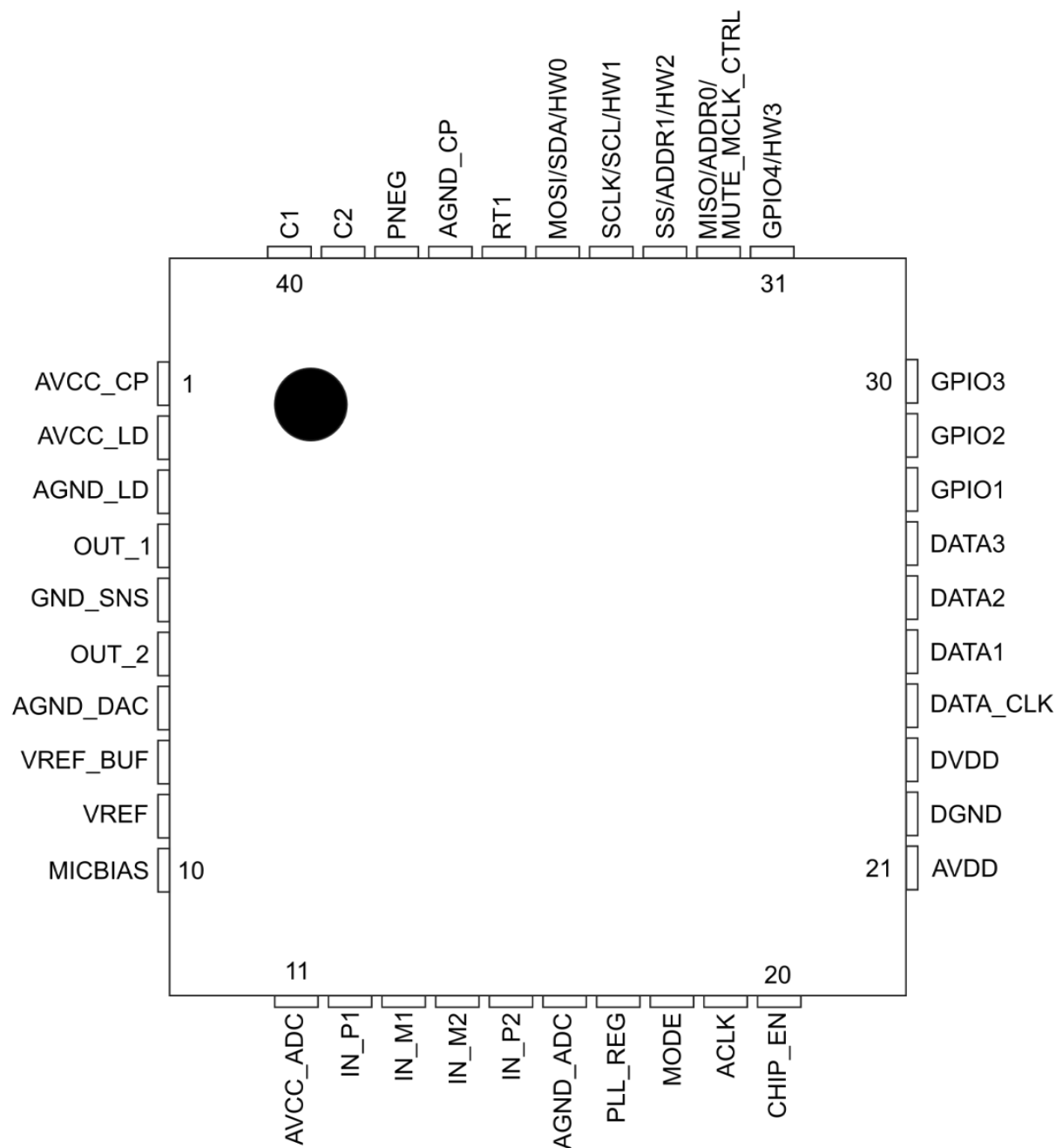
ES9290 (Top View)
