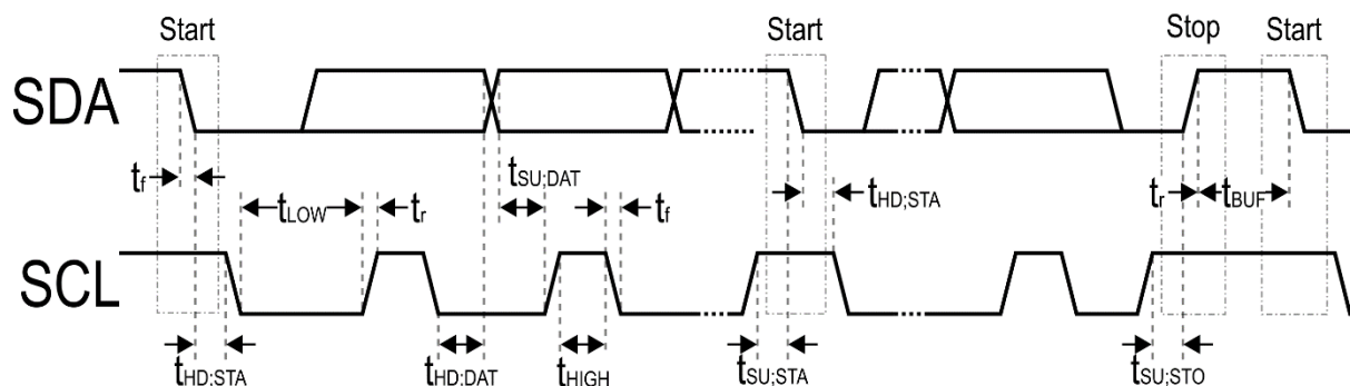
Figure 6 - I 2 C Slave Control Interface Timing
