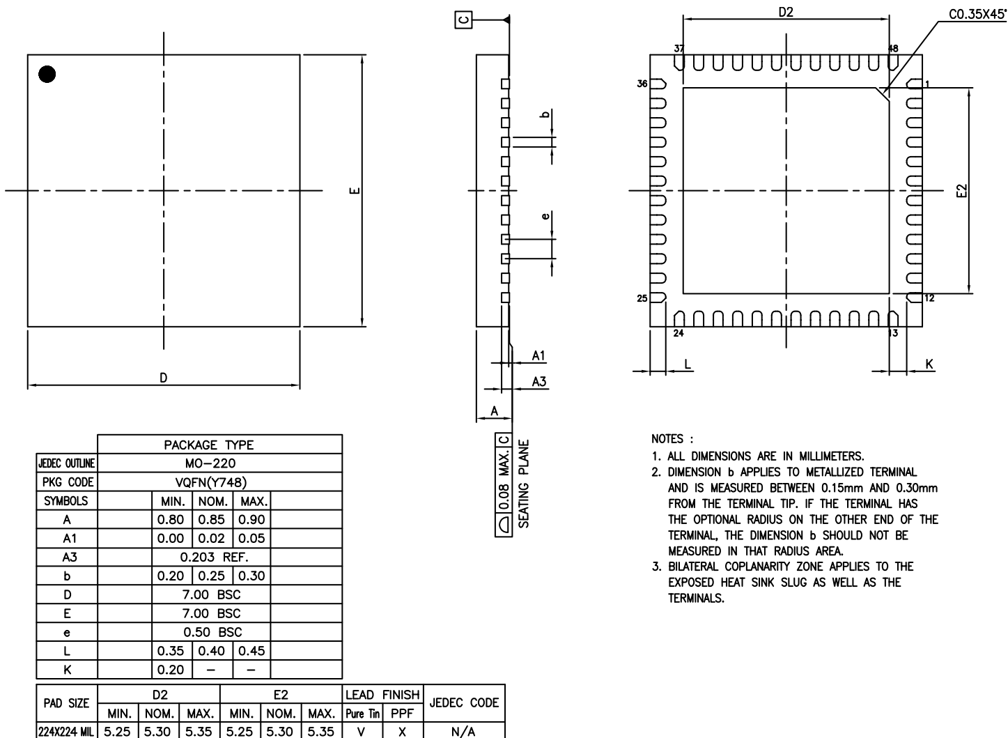
Figure 32 - ES9017Q 48 QFN Package Dimensions
