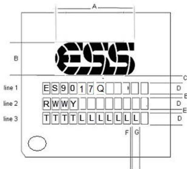
Figure 34 - ES9017Q Marking
