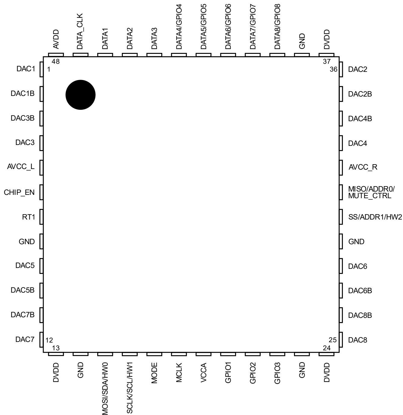
Figure 2 - 48 QFN/QFP Pinout
