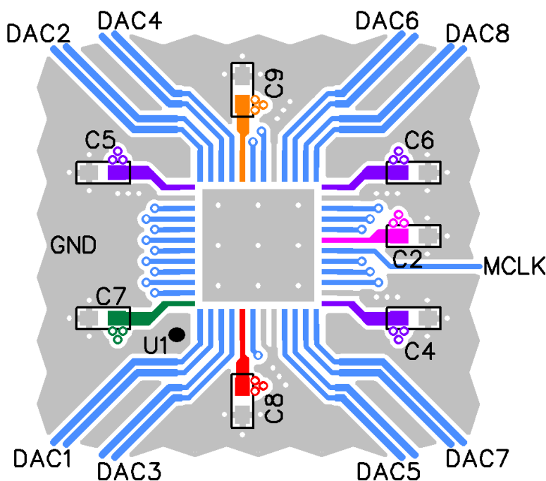
Figure 30 - ES9017 Recommended PCB Layout Guidelines
