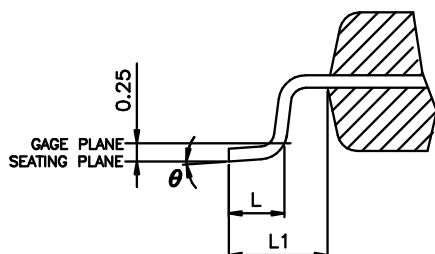
Figure 31 - ES9017S 48 QFP Package Dimensions
