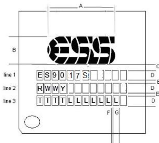
Figure 33 - ES9017S Marking
