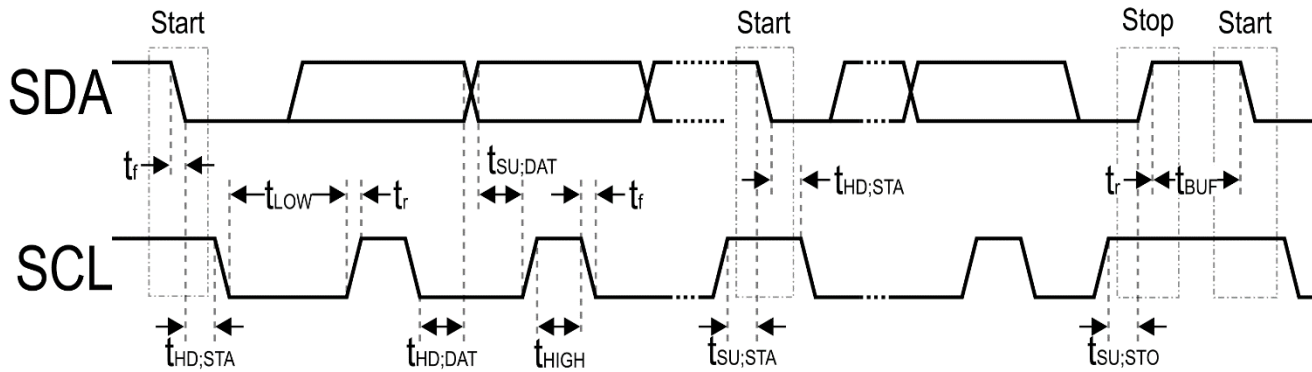
Figure 22 - I 2 C Slave Control Interface Timing
