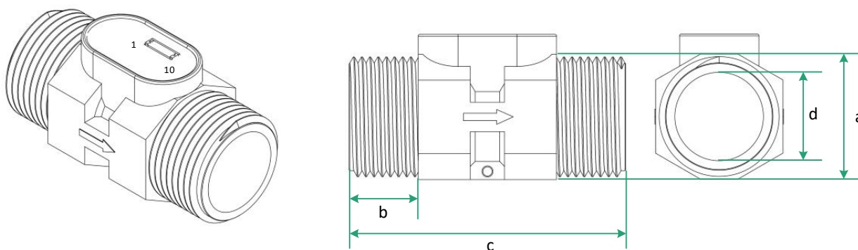
Figure 2: Mechanical drawings
